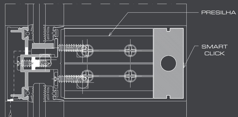
CORTE VERTICAL
